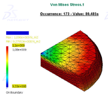
Figure 2- Distribution of Von Mises's stress (displacement of die 8 mm )
