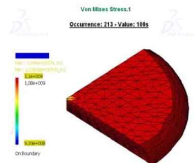
Figure 3 - Distribution of Von Mises's stress (displacement of die 10 mm )
